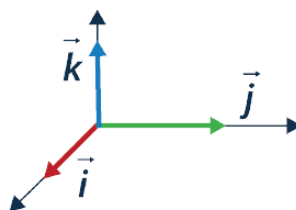
3D Vectors
