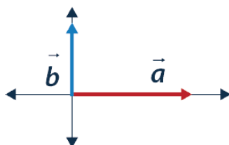
2D Vectors
