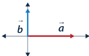
2D Vectors
