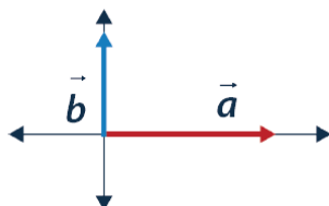
2D Vectors
