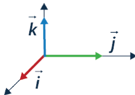
3D Vectors
